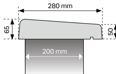
COUVERTINE 1 PENTE
