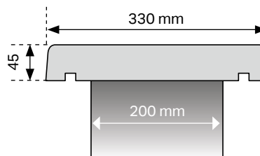
COUVERTINE PLATE
